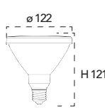
Lampadina a Led 18W, 240V
